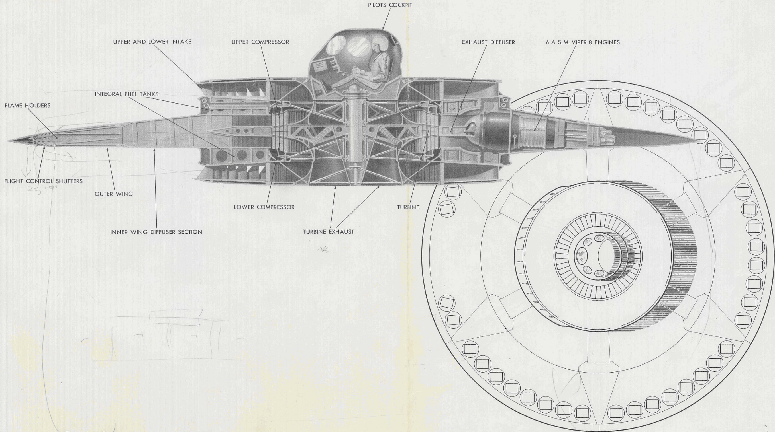
Fig. 1 Plan view and section through aircraft
