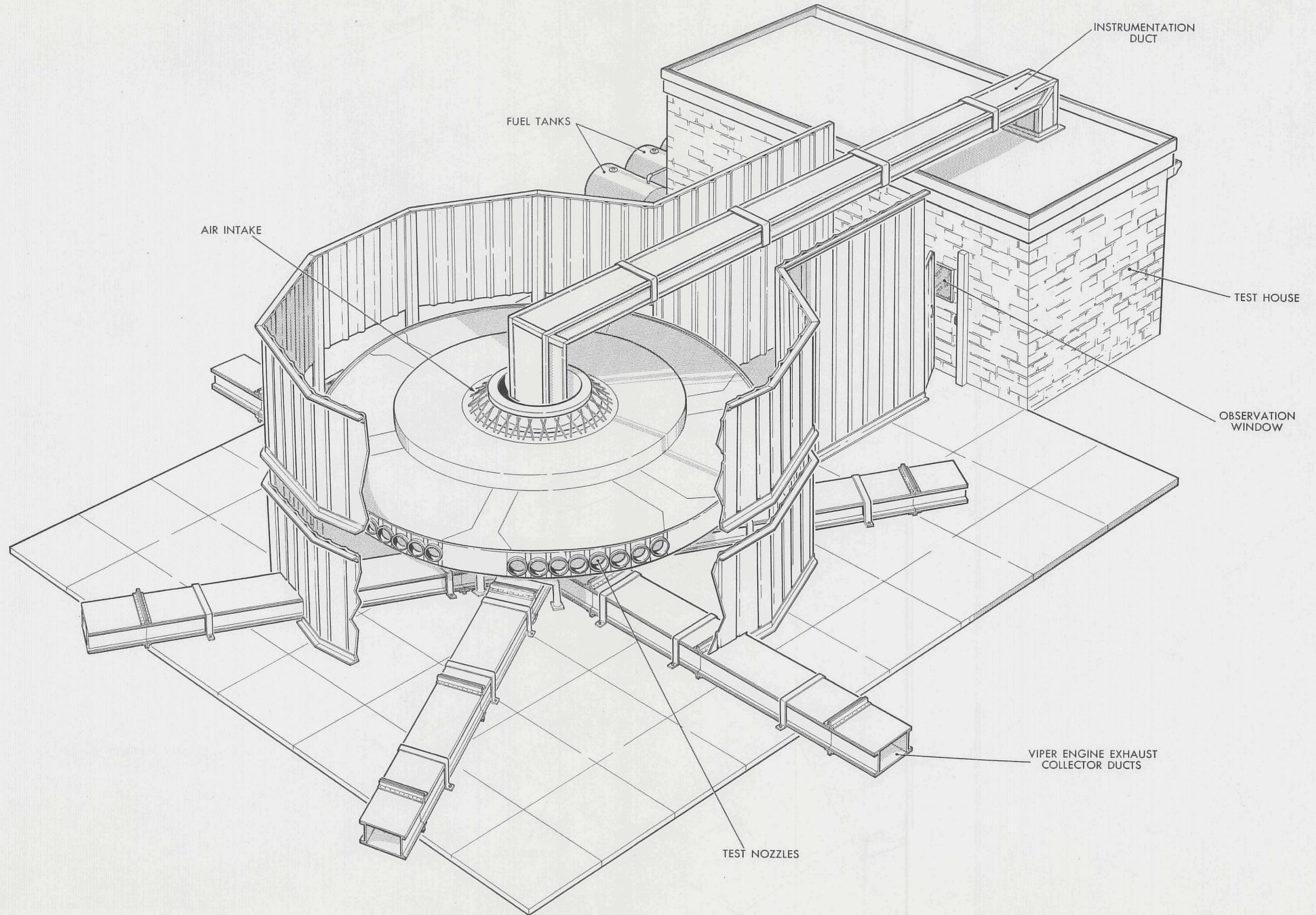
FIG.40 TEST HOUSE AND SIX VIPER TEST RIG
