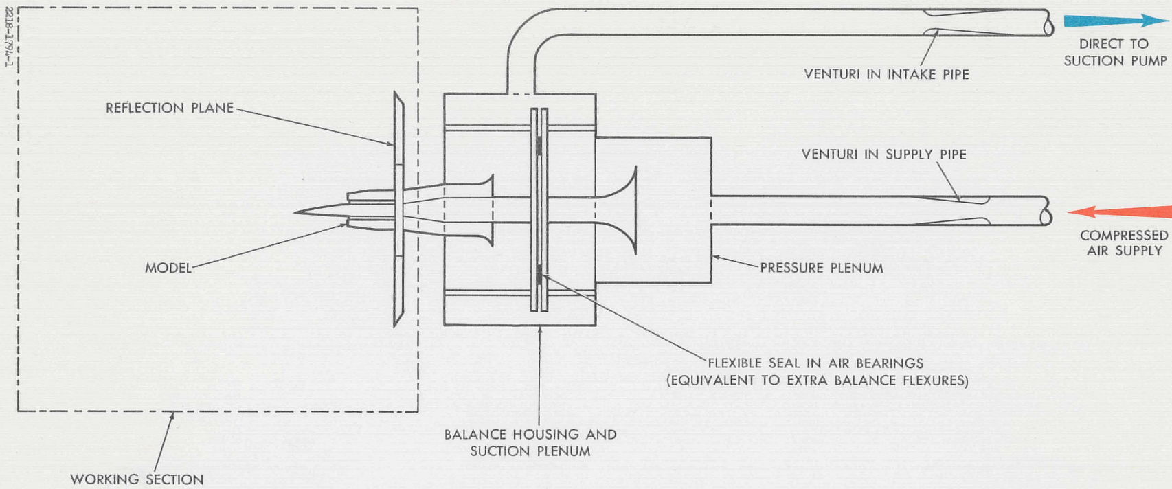
FIG. 23 PROPOSED CHANGES TO 1/23 SCALE MODEL
