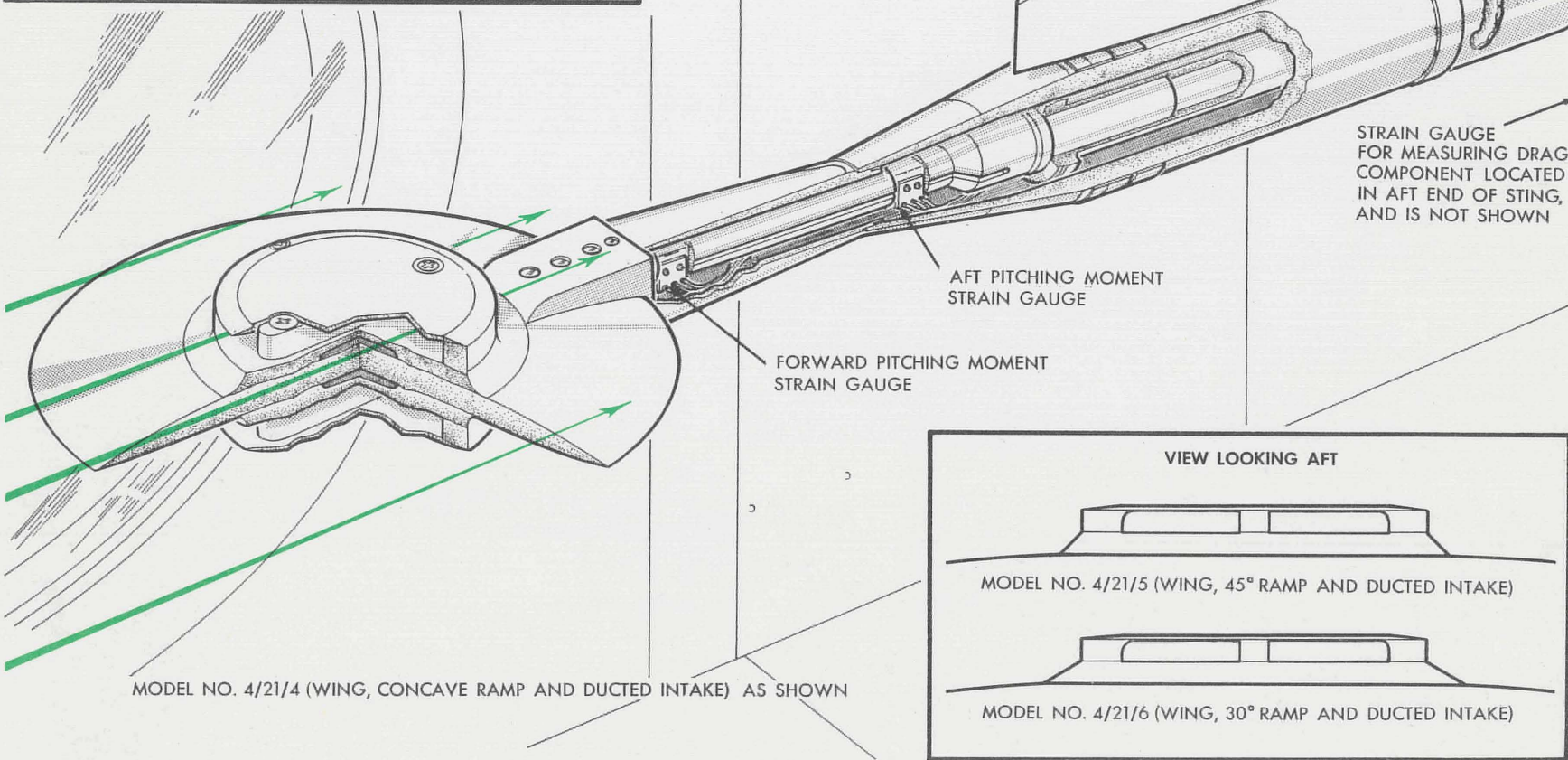
FIG. 20 1/40 SCALE STING MOUNTED MODEL
