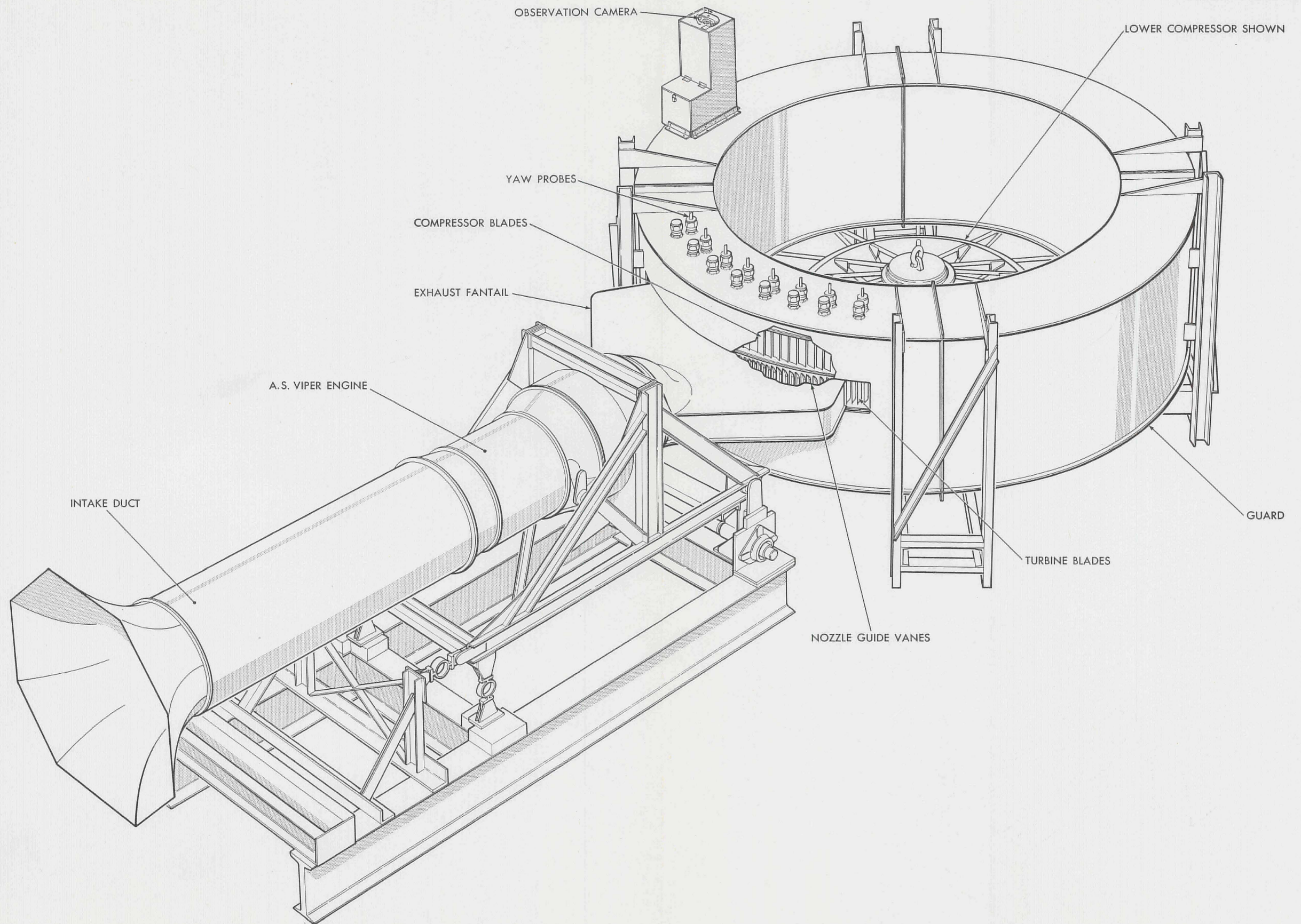
FIG. 39 BALANCE AND OVERSPEED RIG
