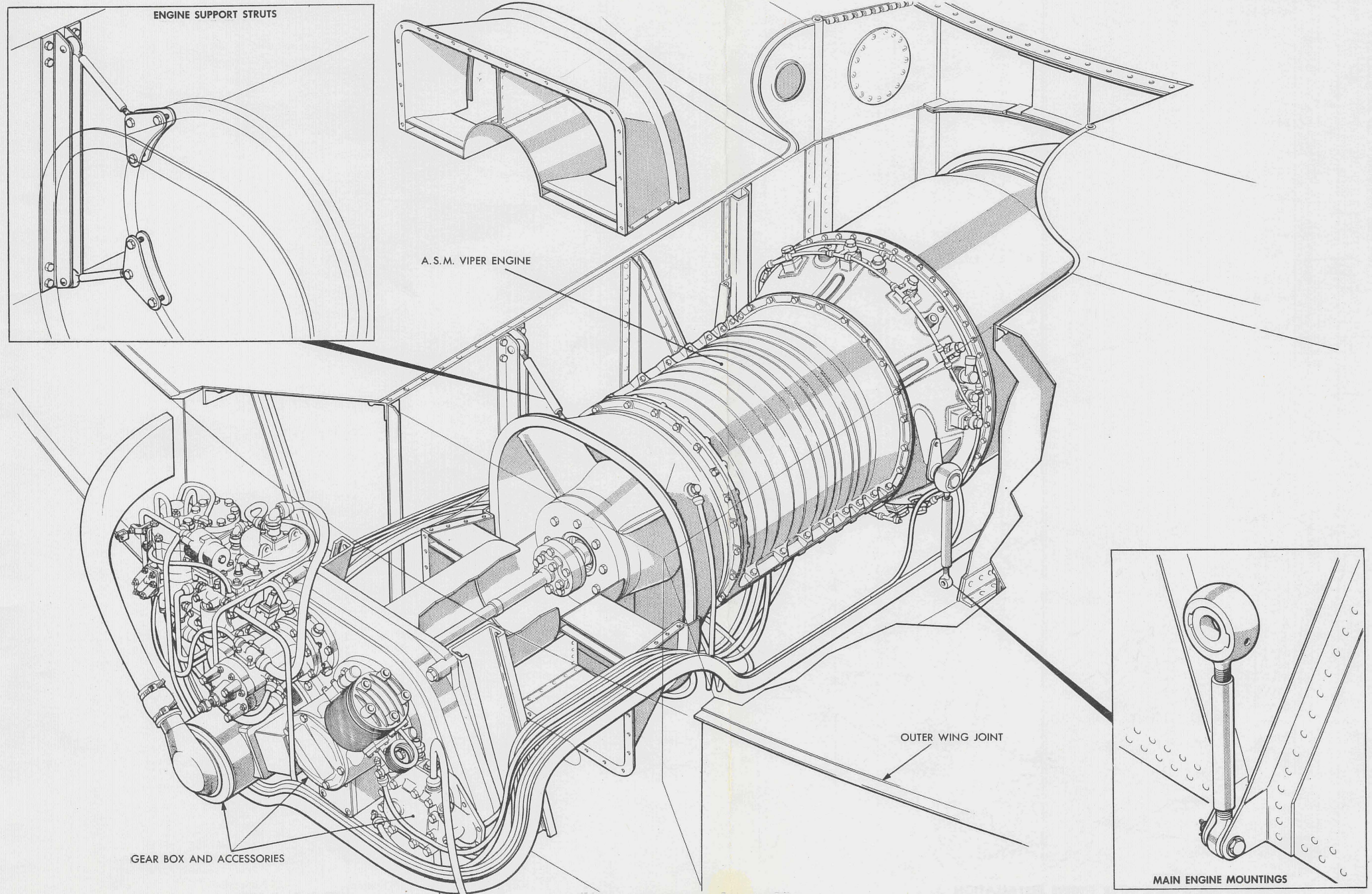
FIG. 4 A.S. VIPER ENGINE INSTALLATION
