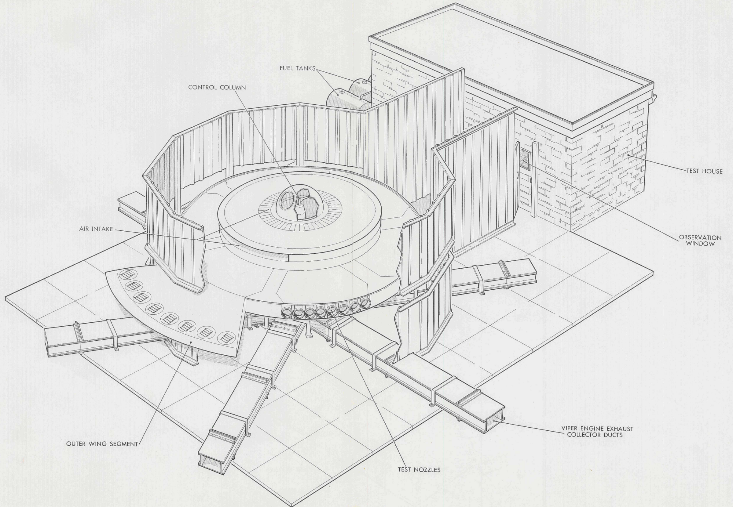
FIG. 44 SIX VIPER TEST RIG WITH OUTER WING AND COCKPIT
