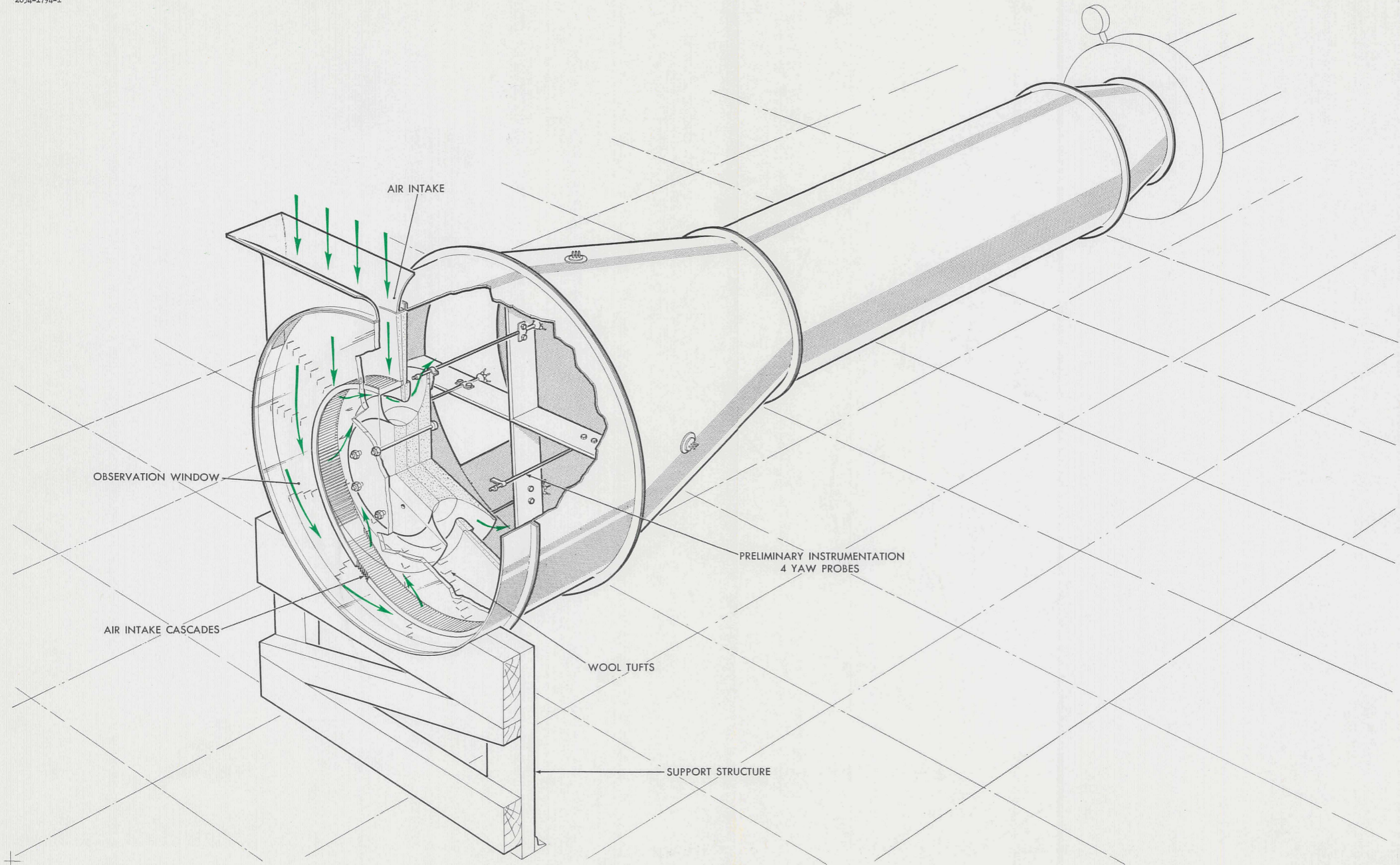
FIG. 26 1/5th SCALE AIR INTAKE MODEL
