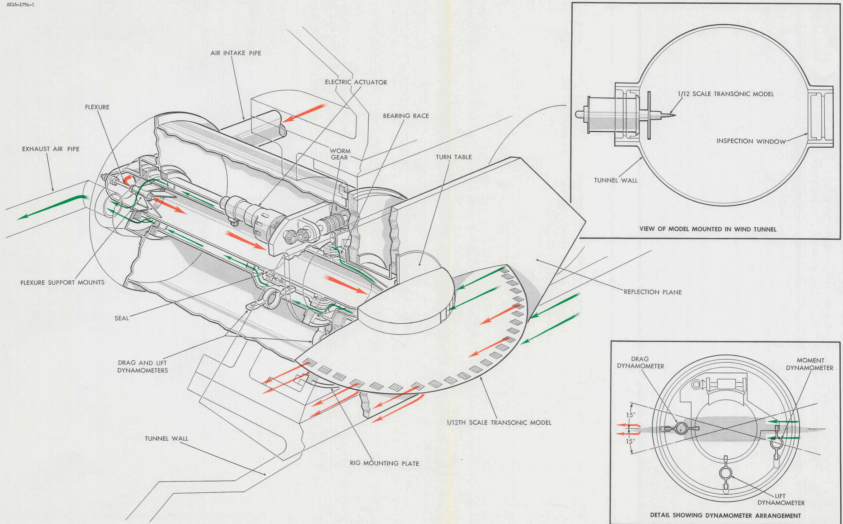
FIG. 14 PROPOSED 1/12TH SCALE TRANSONIC REFLECTION PLANE MODEL
