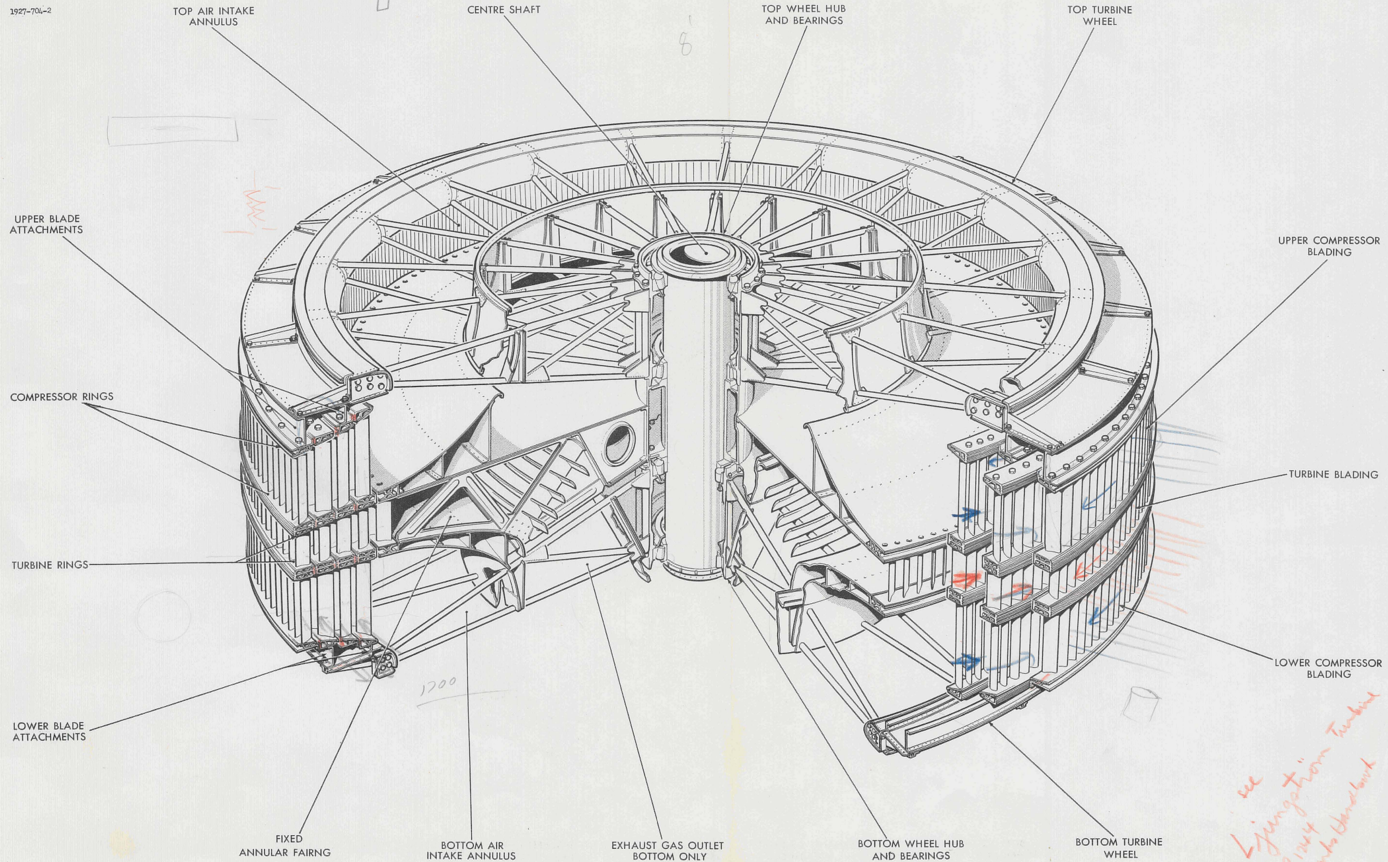
FIG. 3 TURBINE-COMPRESSOR ASSEMBLY
