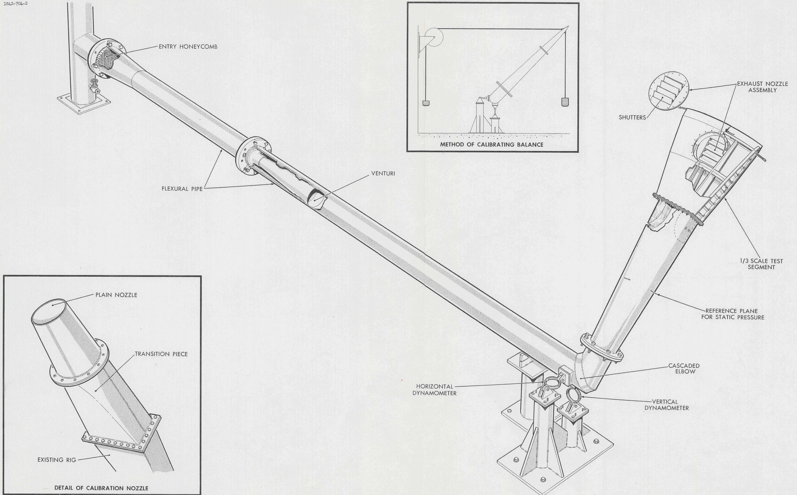
FIG. 25 1/3 SCALE OUTER WING SEGMENT TEST RIG
