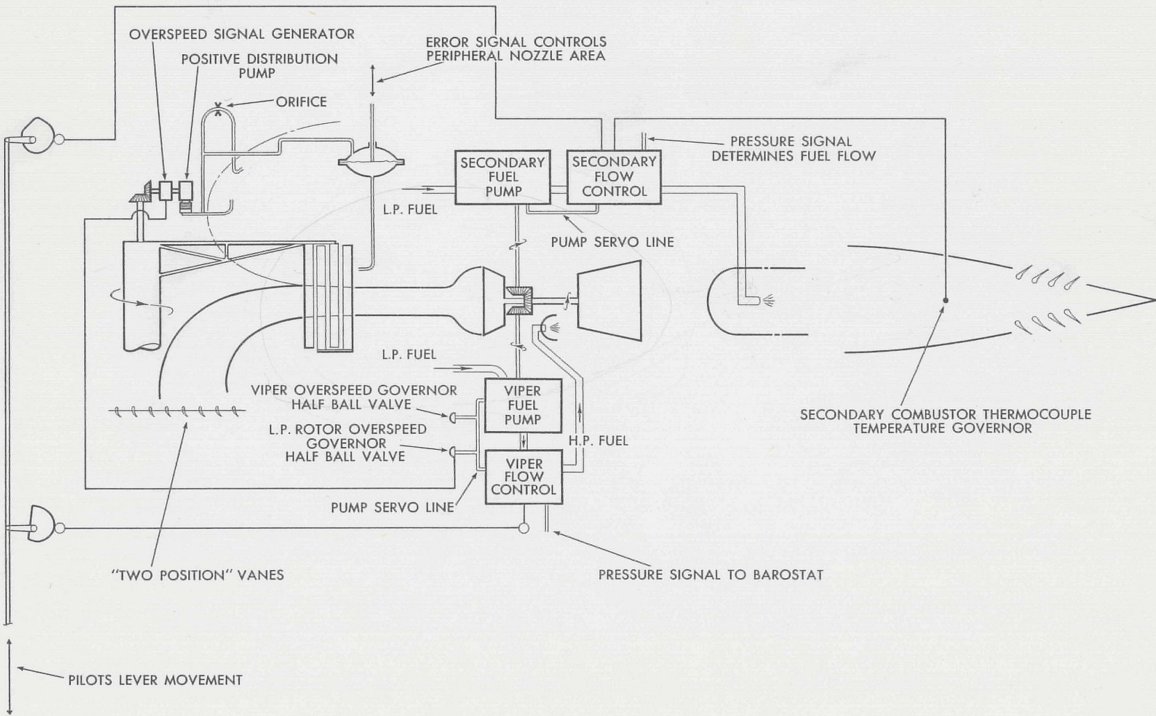
FIG. 34 SCHEMATIC OF PROPUSION CONTROL SYSTEM
