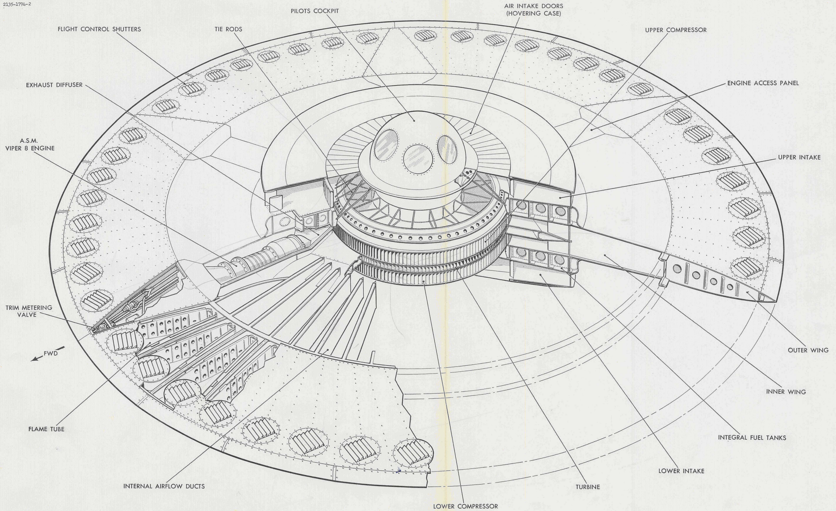
FIG. 2 CUTAWAY OF AIRCRAFT STRUCTURE
