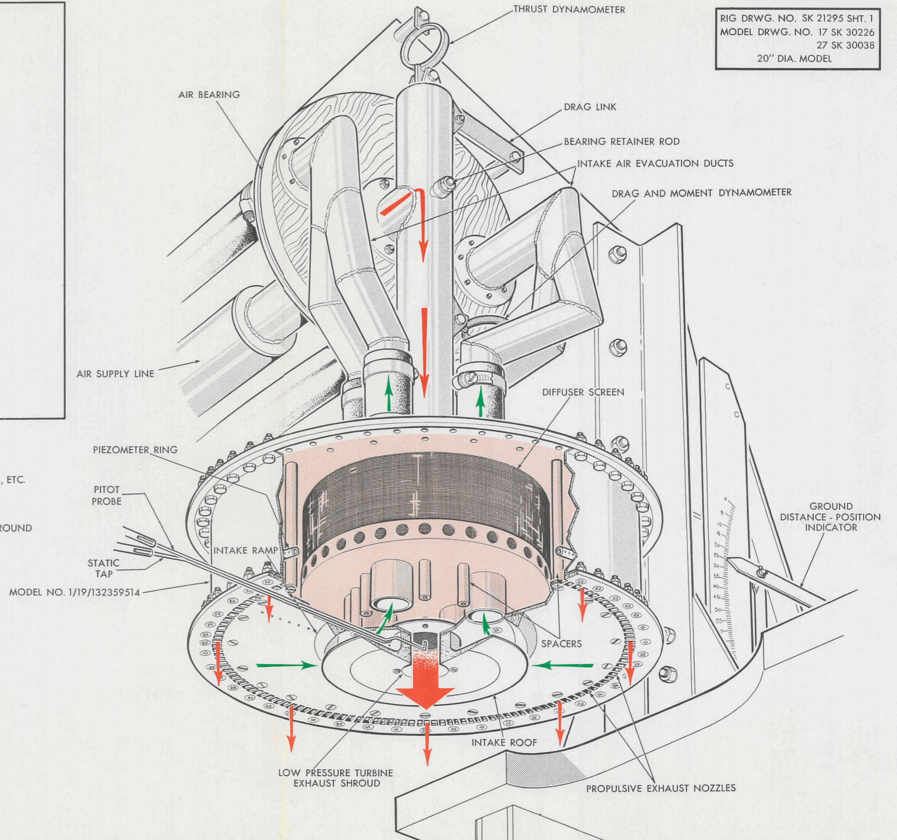
FIG. 29 GROUND EFFECTS RIG
