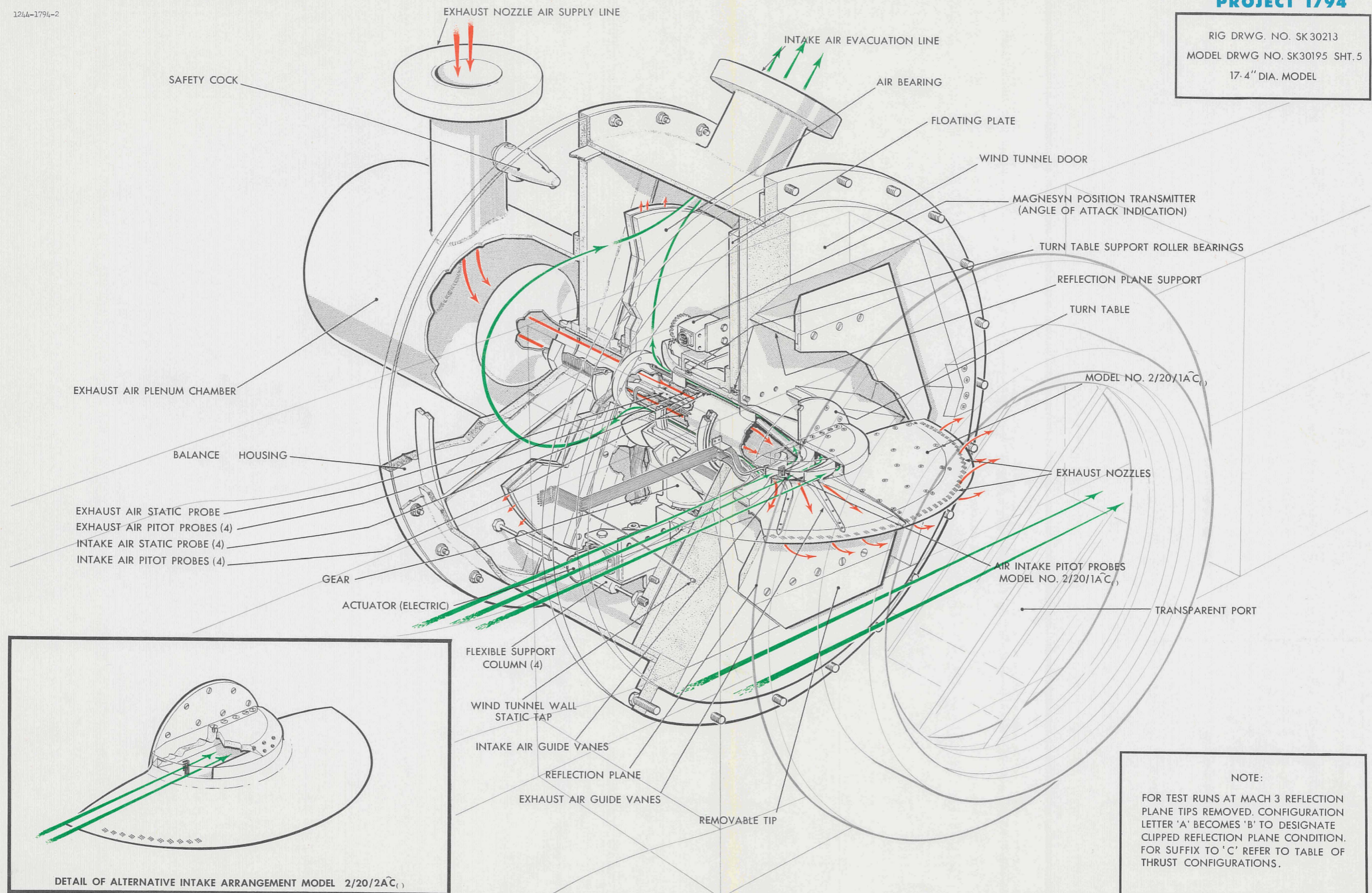
FIG. 22 1/23 SCALE SUPERSONIC MODEL
