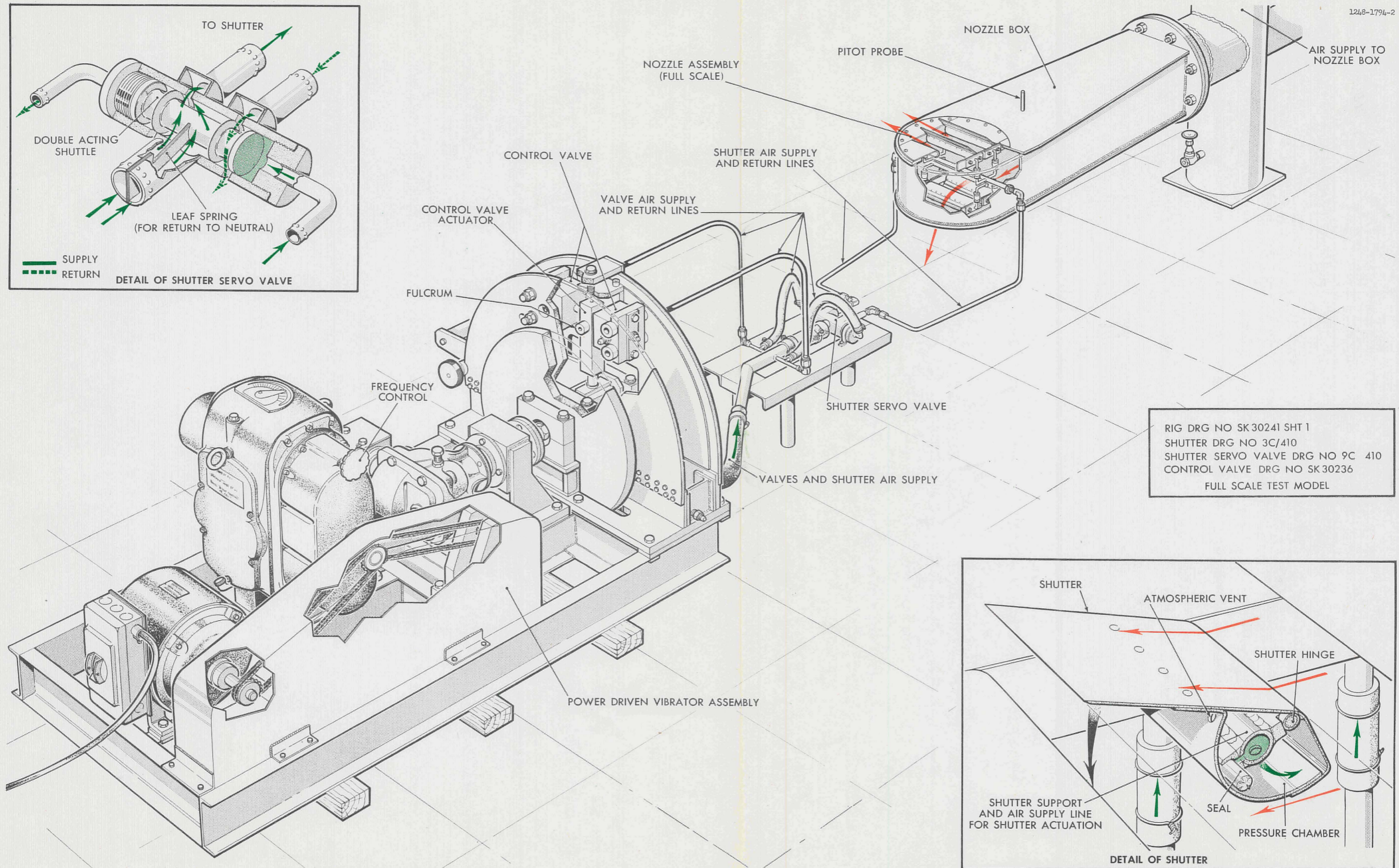
FIG. 51 FREQUENCY RESPONSE RIG NO. 1
