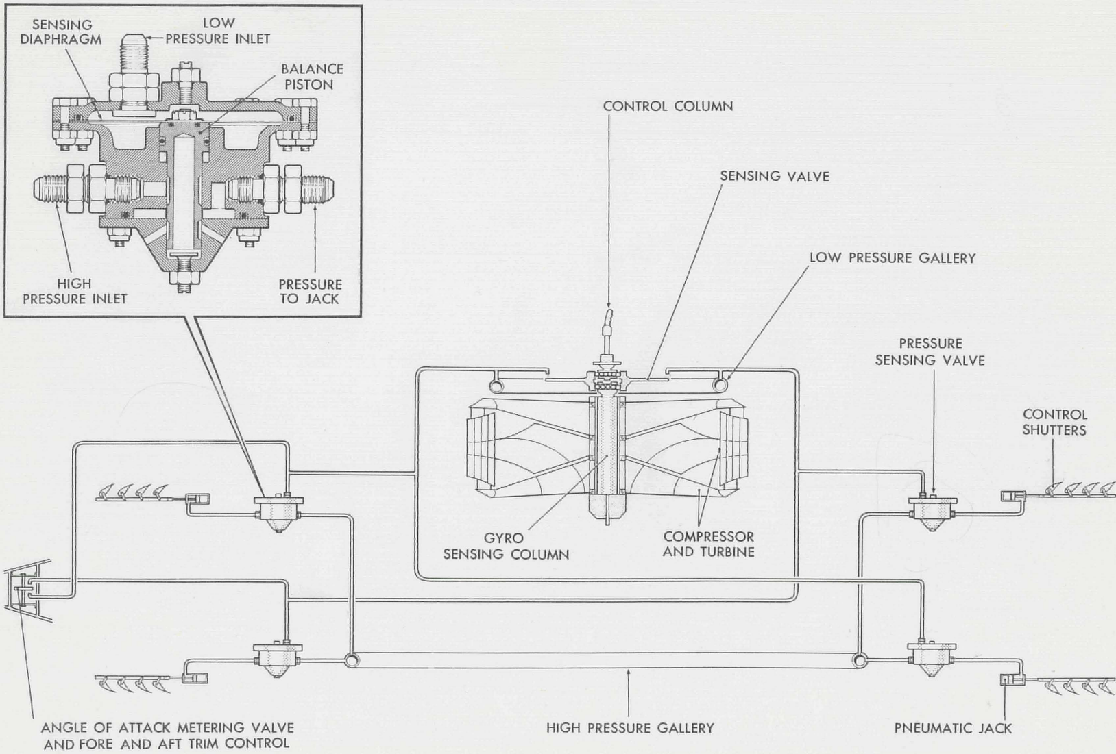
FIG.49 SCHEMATIC OF SHUTTER CONTROL SYSTEM
