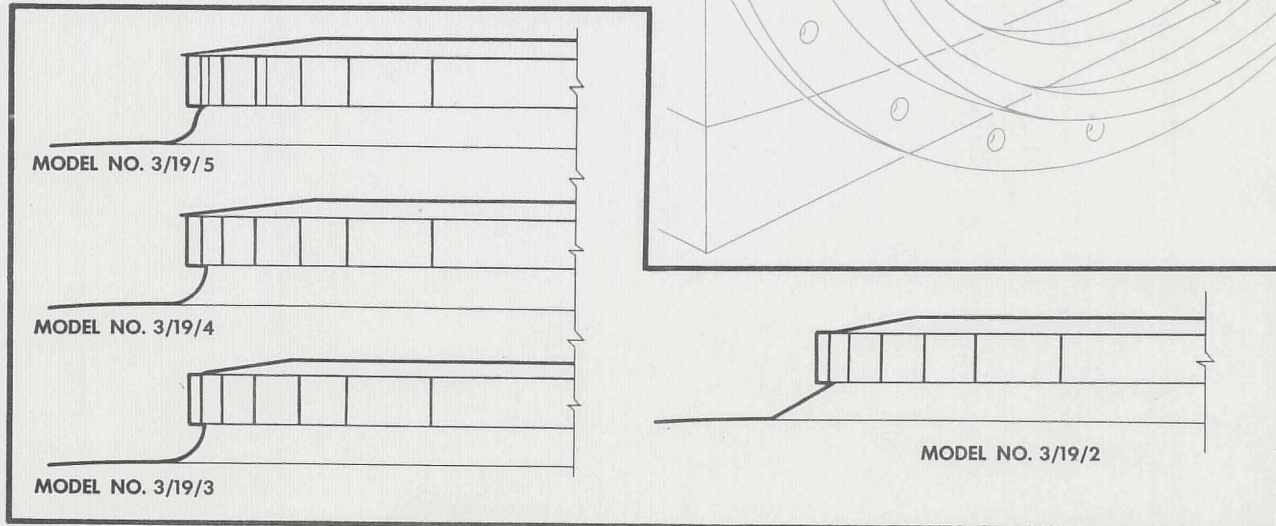
FIG. 16 2/25 SCALE AIR INTAKE MODEL
