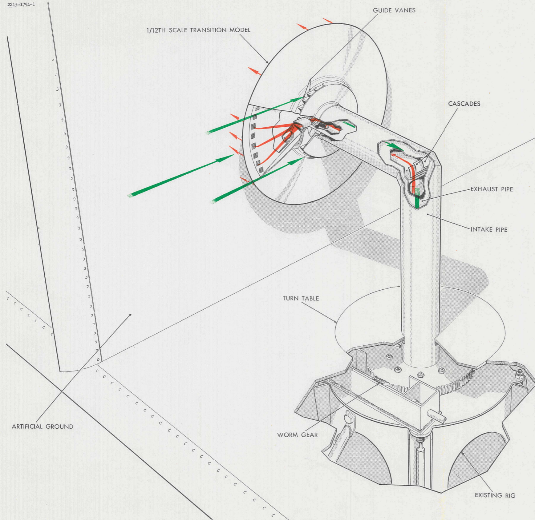
FIG. 11 PROPOSED 1/12TH SCALE TRANSITION MODEL
