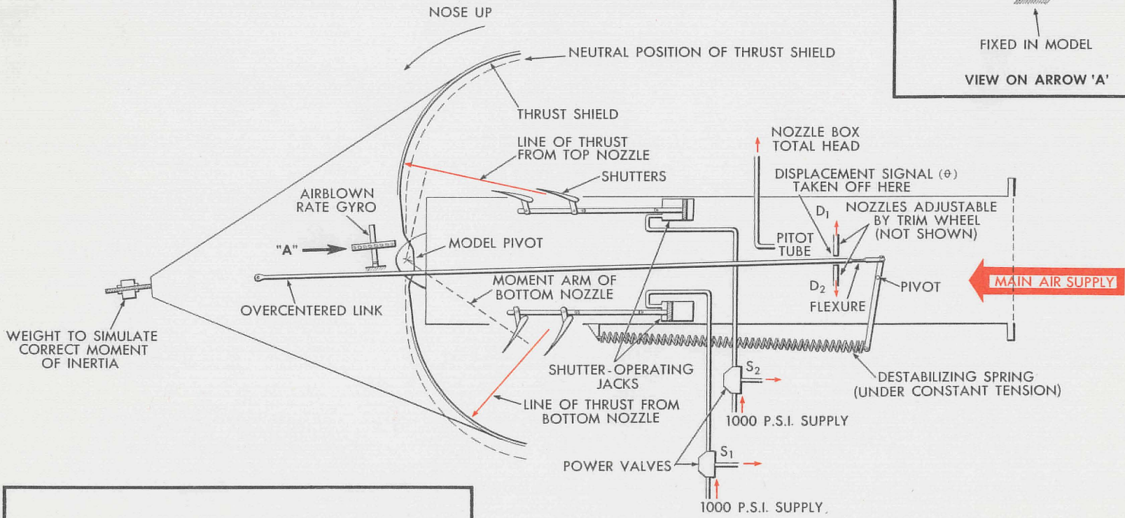
FIG. 52 SCHEMATIC OF CONTROL SYSTEM MECHANICAL ANALOG
