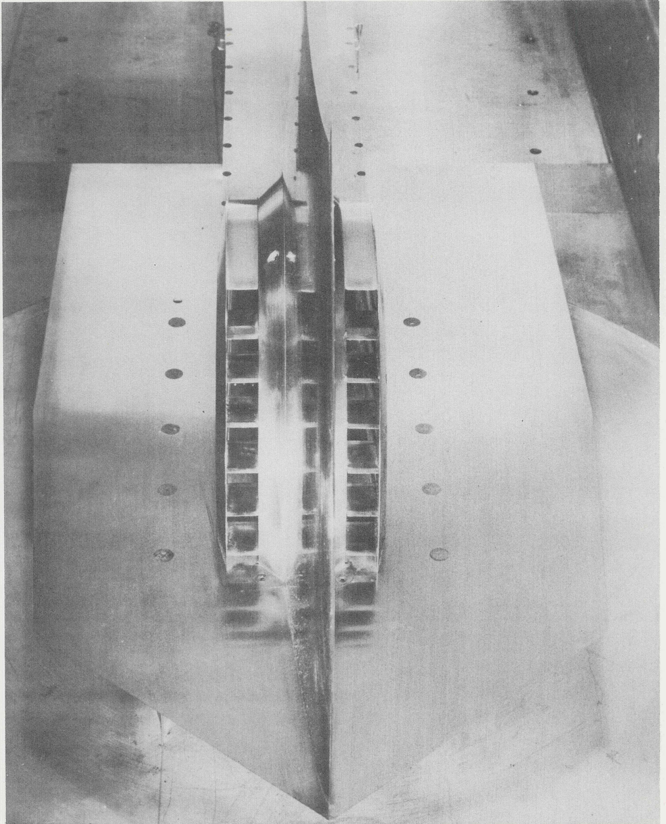
FIG. 15 2/25 SCALE AIR INTAKE MODEL
